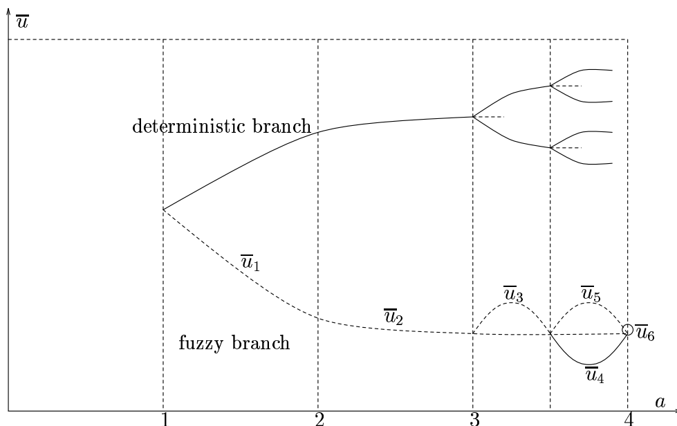
FIGURE 2. Bifurcation Diagram
