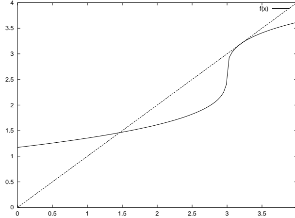
FIGURE 1. Fixed Points of f(x)
