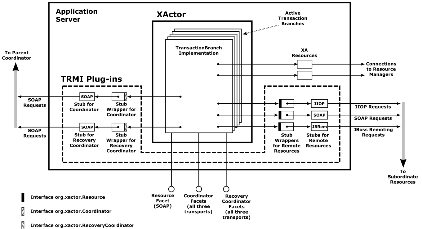
Figure 3: A TransactionBranch instance within XActor.
