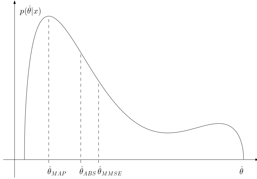
Fig. 4.2 A posterior density p(\theta | \mathbf{x}) , and the respective MAP estimate \hat{\theta}_{MAP} , minimum MSE estimate \hat{\theta}_{MSE} , and the minimum absolute error estimate \hat{\theta}_{ABS} .
