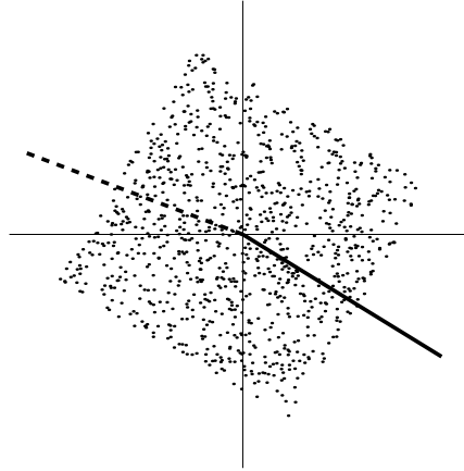
Fig. 8.16 Result of FastICA using kurtosis, for ICs with uniform distributions. Dashed line: \mathbf{w} after the first iteration (plotted longer than actual size). Solid line: \mathbf{w} after the second iteration.
