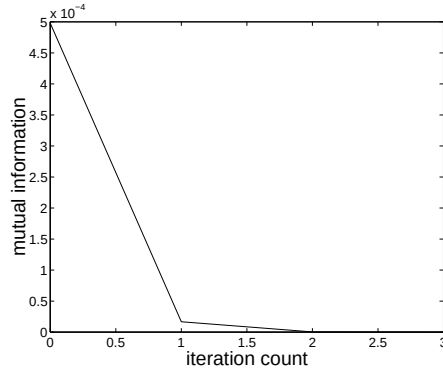
Fig. 10.1 The convergence of FastICA for ICs with uniform distributions. The value of mutual information shown as function of iteration count.
