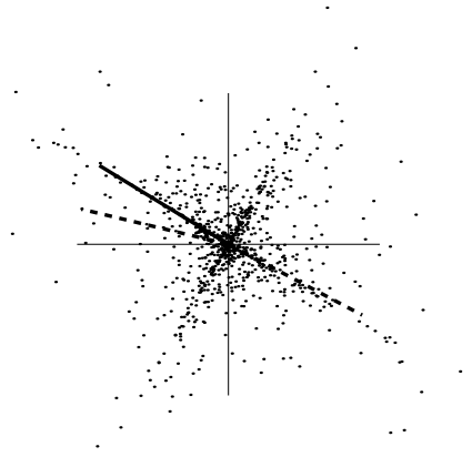
Fig. 8.24 Results with FastICA using negentropy, second experiment. Dashed line: \mathbf{w} after the first iteration (plotted longer than actual size). Solid line: \mathbf{w} after the second iteration.
