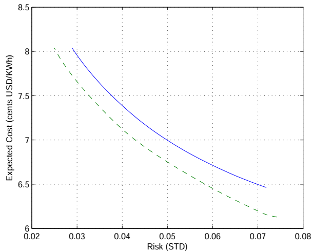
Figure 3: Efficient frontier for the nominal data (dashed line) and the robust problem (13) with ellipsoidal uncertainty set for r (solid line)
