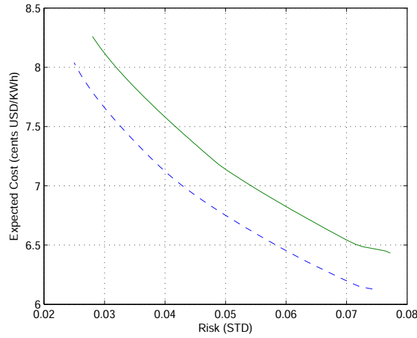
Figure 2: Efficient frontier for the nominal data (dashed line) and the high CO_2 emission cost data (solid line)
