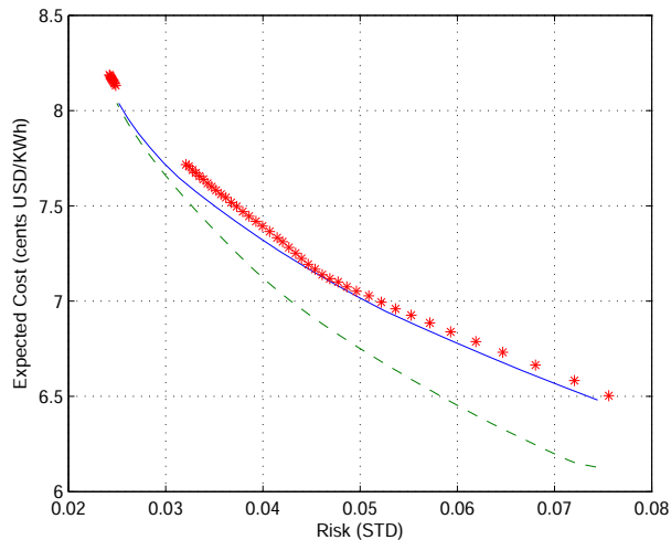
Figure 1: Efficient frontier for the nominal data (dashed line), the robust data for problem (14) (solid line), and robust data for problem (16) (star line)
