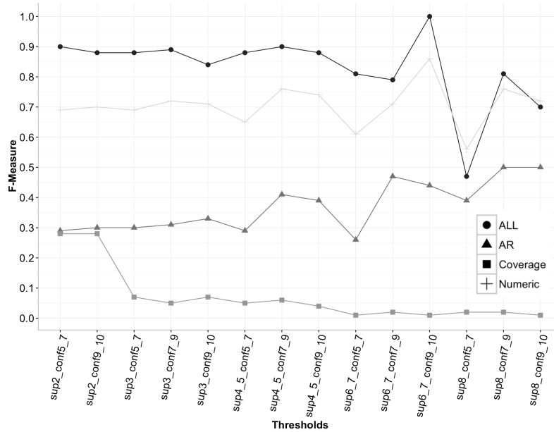
Figure 3. Average F-measure values to predict co-changes by thresholds of support and confidence
