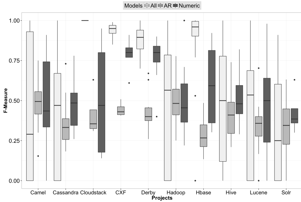
Figure 2. F-measure values to predict co-changes by project considering all releases
