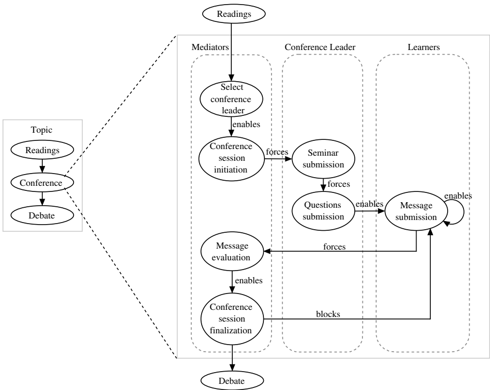
Fig. 9. ITAE conference coordination protocol.
