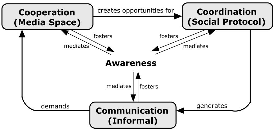
Fig. 1. 3C collaboration model instantiated for the Media Space domain.
