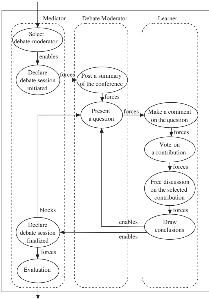
Fig. 16. ITAE debate coordination protocol.
