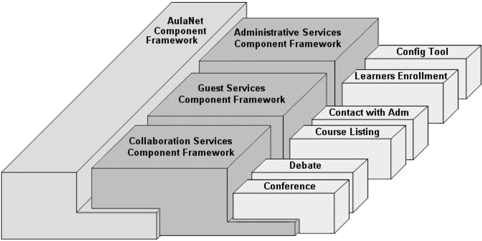
Fig. 13. AulaNet's system architecture (for the sake of clarity only a few services were listed).
