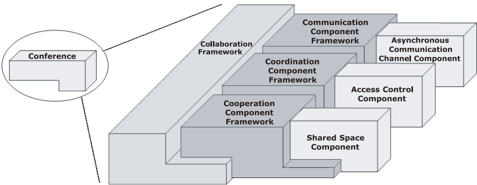
Fig. 14. Architecture of a collaboration service.
