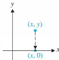
Figure 3.11 A projection
