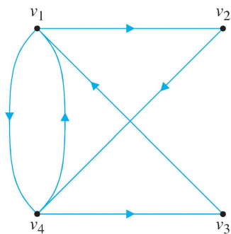
Figure 3.26 A digraph
