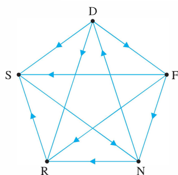
Figure 3.27 A tournament
