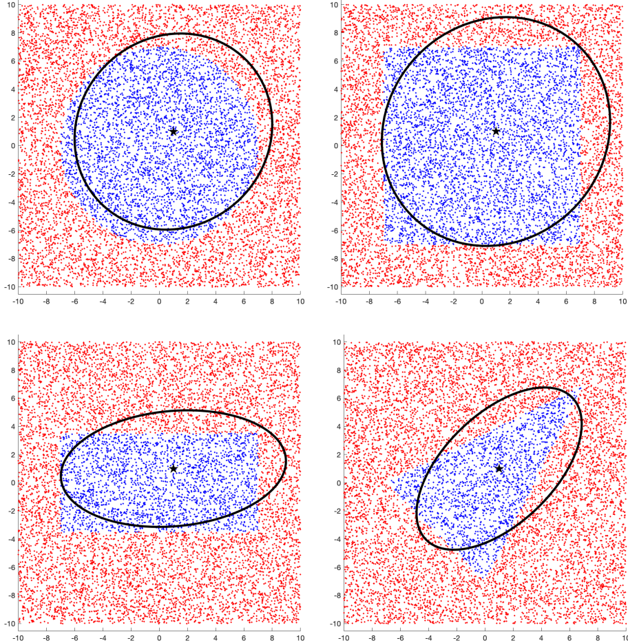
Figure 4: Illustration of the solutions obtained by Algorithm 1 for different smoothing functions in solving the four instances of the classification problem (41). The center of each ellipse is marked with a star.
