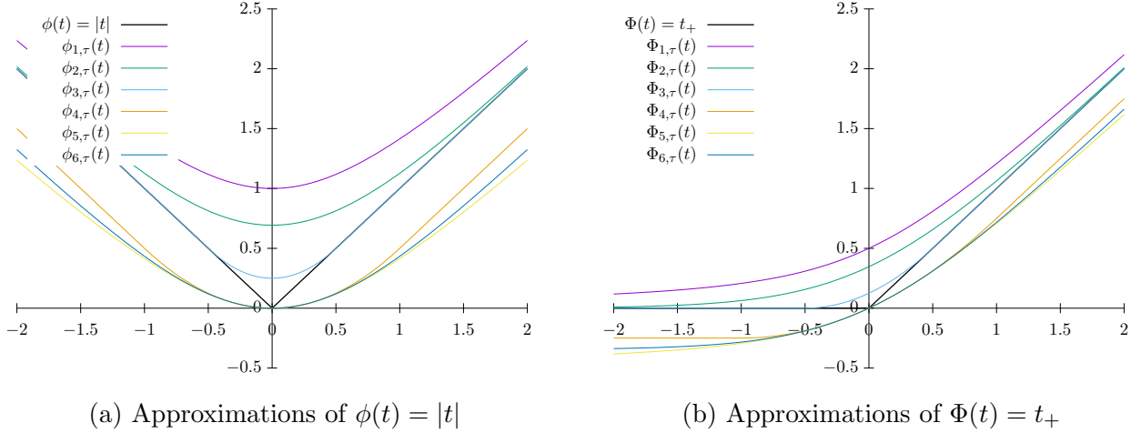
Figure 1: Approximations of \phi(t) = |t| and \Phi(t) = t_+ as described in Example 2.
