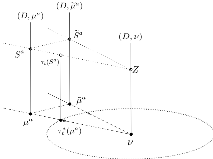
FIGURE 1. Action of the scaling flow on the fiber bundle \mathcal{M}_F \times D : since \nu is a fixed point, \tau_t moves Z within its fiber (D, \nu) , with the dotted lines indicating part of its Cesáro stable manifold.
