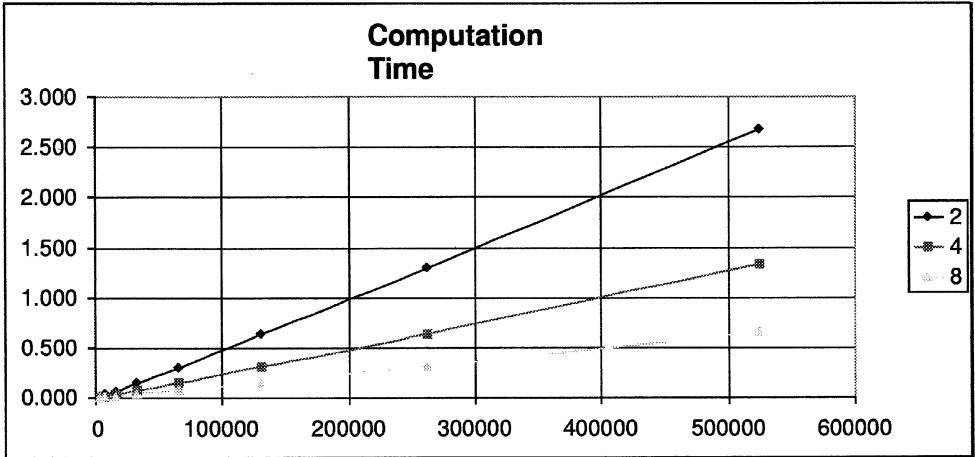
Figure 1: Computation Times (In Seconds) For Different Numbers Of Data Items. The Three Curves Represent Configurations Of 2, 4, And 8 Processors, Respectively.
