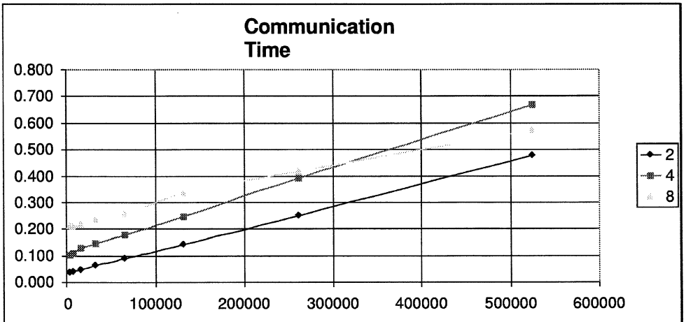
Figure 2: Communication Times (In Seconds) For Different Numbers Of Data Items. The Three Curves Represent Configurations Of 2, 4, And 8 Processors, Respectively.
