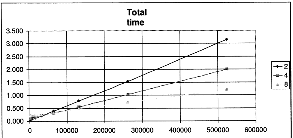
Figure 3: Total Running Times (In Seconds) For Different Numbers Of Data Items. The Three Curves Represent Configurations Of 2, 4, And 8 Processors, Respectively.
