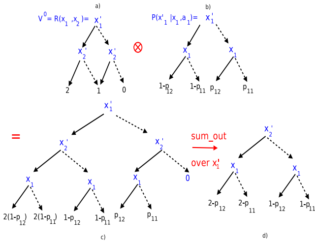
Figure 3: a) We show V_{ADD}^0 = R(x_1, x_2) = \sum_{i=1}^2 x_i represented as an ADD. b) The PADD representation for \bar{P}(x'_1|x_1, a_1) ( CPT_{a_1}^{x'_1} ). c) The multiplication V_{ADD}^0 \otimes CPT_{a_1}^{x'_1} resulting in a PADD. d) The result of summing out over x'_1 , which is a PADD.
