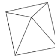
octahedron (wind)
