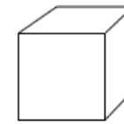
hexahedron (cube) (earth)
