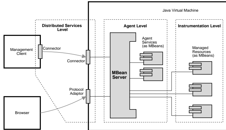
Fig. 1. The JMX architecture
