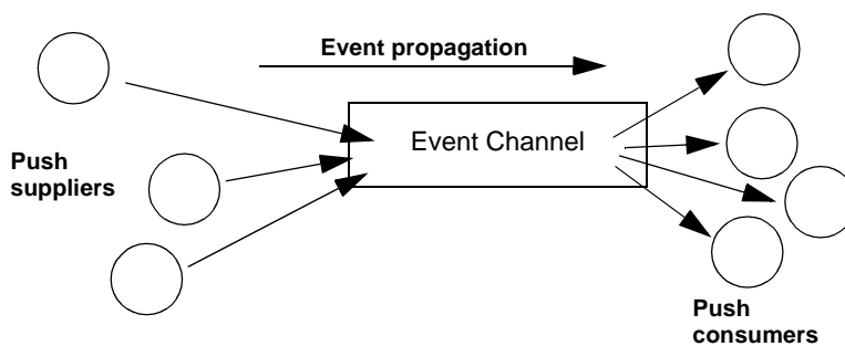
Figure 35: Push model of event transfer
